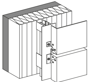
2 CASSETTE SCREWED for vertical façade structuring
